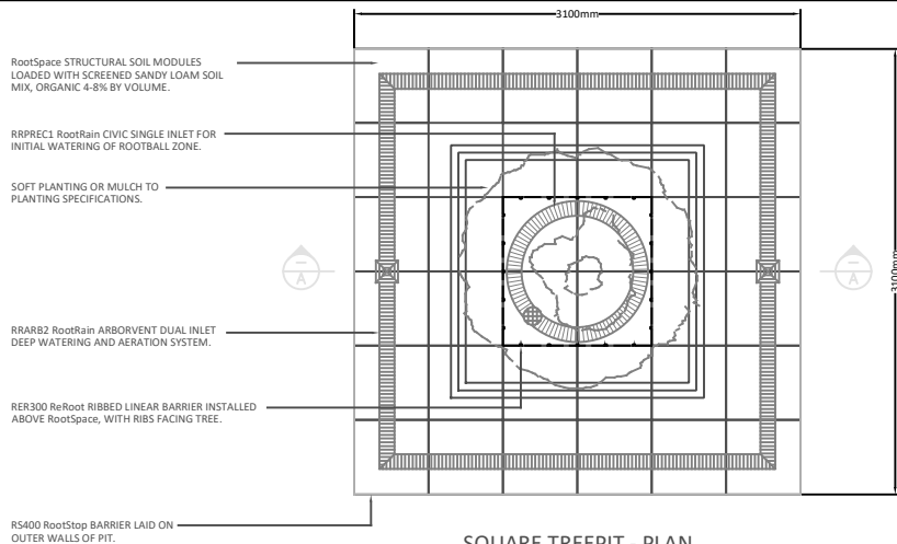
SQUARE TREEPIT - PLAN
